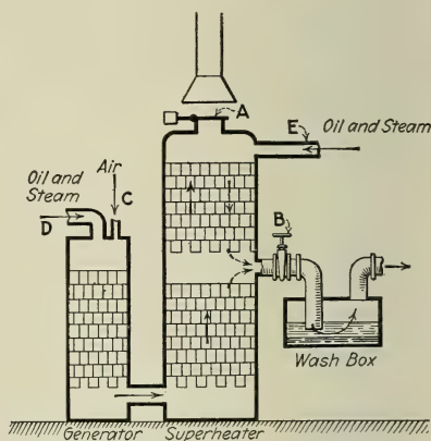
FIG. 103.—Oil-water Gas Plant.
